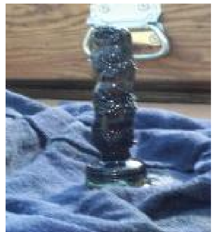
Below: The FilterMaster 2000 Series Magnetic Filter Rod, in service on the same gear box for only 37 days.
